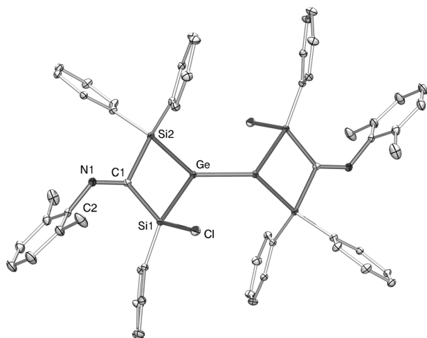
Figure 2. Crystal structure of 5 (thermal ellipsoids at 30%, isopropyl groups of aryl substituted, hydrogen atoms, and benzene molecule as solvent are omitted for clarity). Selected bond lengths [ \text{\AA} ] and angles [ ^\circ ]: \text{Ge}-\text{Ge} 2.2944(4) , \text{Ge}-\text{Si}1 2.4126(5) , \text{Ge}-\text{Si}2 2.4518(5) , \text{Si}1-\text{C}1 1.9410(17) , \text{Si}2-\text{C}1 1.9666(17) , \text{N}1-\text{C}1 1.272(2) , \text{N}1-\text{C}2 1.419(2) ; \text{Ge}'-\text{Ge}-\text{Si}1 122.236(16) , \text{Ge}'-\text{Ge}-\text{Si}2 131.336(17) , \text{Si}1-\text{Ge}-\text{Si}2 80.950(16) , \text{C}1-\text{Si}1-\text{Ge} 85.52(5) , \text{C}1-\text{Si}2-\text{Ge} 83.90(5) , \text{C}1-\text{N}1-\text{C}2 126.93(15) , \text{N}1-\text{C}1-\text{Si}1 132.91(13) , \text{N}1-\text{C}1-\text{Si}2 116.88(13) , \text{Si}1-\text{C}1-\text{Si}2 107.81(8) .
