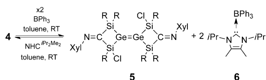
Scheme 5. Reversible reaction of 4 with triphenylborane under formation of digermene 5 (R=Tip).
