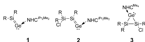
Scheme 2. Heavier vinylidenes 1 and 2 as well as cyclopropylidene analogue 3 ( R = \text{Tip} = 2,4,6\text{-}i\text{Pr}_3\text{C}_6\text{H}_2 , \text{NHC}^{i\text{Pr}_2\text{Me}_2} = 1,3\text{-diisopropyl-4,5-dimethylimidazol-2-ylidene} , \text{NHC}^{\text{Me}_4} = 1,3,4,5\text{-tetramethylimidazol-2-ylidene} ).
